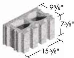
4 Rib: Typical 8" Size
