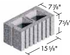
8 Rib: Typical 8" Size
